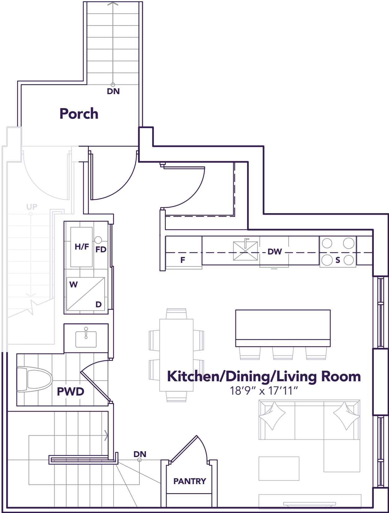
LIVING LEVEL
