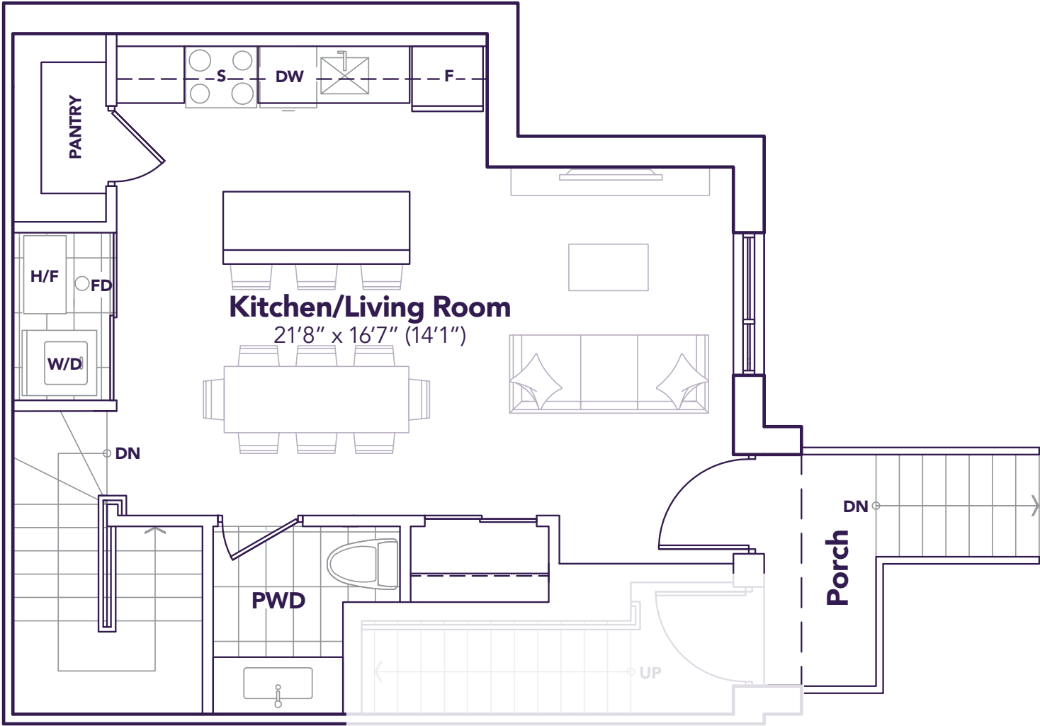
LIVING LEVEL
