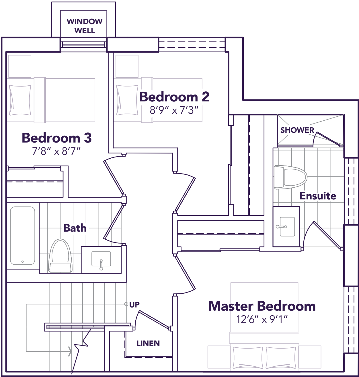
BEDROOM LEVEL
