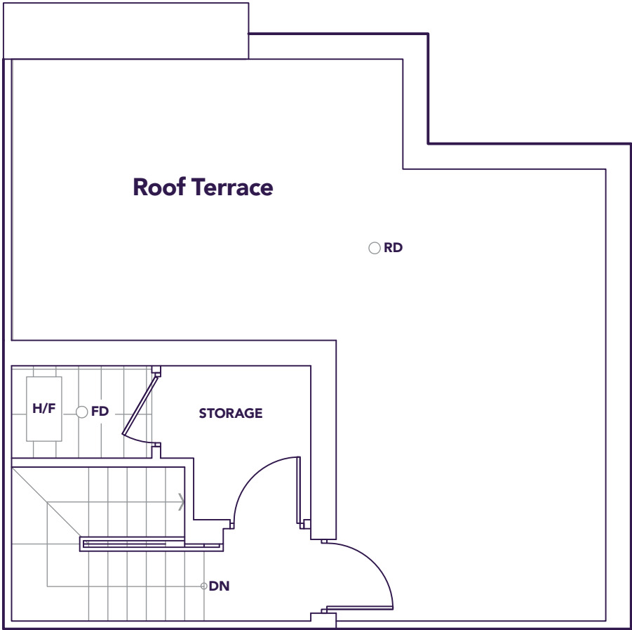
TERRACE LEVEL
